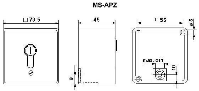
Surface mount key switch, with phc Art.: 107.1101.10
