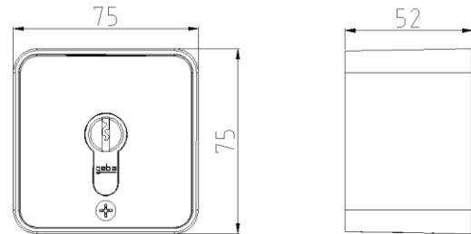
Surface-mount key switch With phc Art.: 009.1202.10
