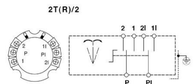
Surface-mount key switch With phc Art.: 009.1202.10
